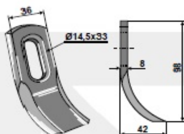
Y-Messer couteau-Y / Y-blade
