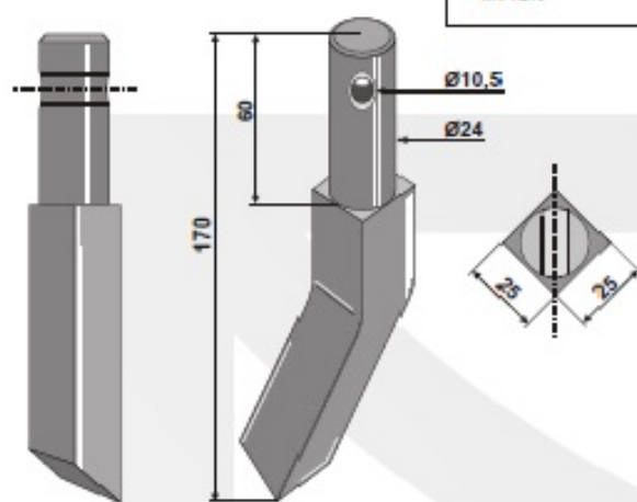
Rotorzinken / dent rotative / rotary tine
